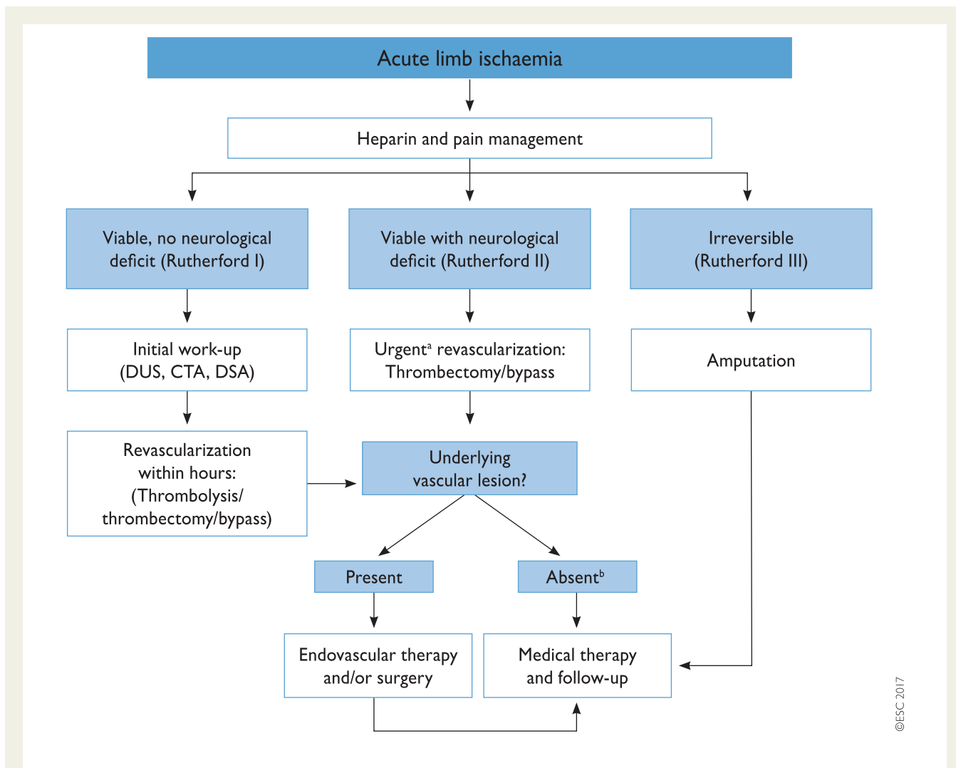
Figure 7 Management of acute limb ischaemia. CTA = computed tomography angiography; DSA = digital subtraction ultrasound; DUS = duplex ultrasound.
